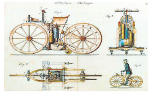
The figures in Reitwagen patent.
